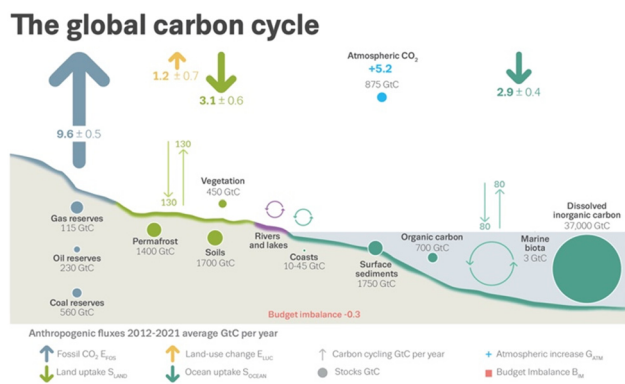
Fig. 1 Schematic representation of the global carbon cycle, highlighting effects from anthropogenic activities averaged globally for the decade 2012–2021. Arrows designate flows. Circles designate reserves. Cyclic arrows designate cycles. Quantities are specified in gigatons of carbon (GtC). The budget imbalance is a measure of imperfect data and understanding of the contemporary carbon cycle. All uncertainties are reported as one standard deviation. Reproduced from Friedlingstein et al. 18
