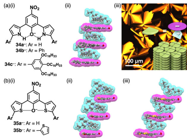
Fig. 21 (a) (i) Deprotonated dipyrrolylnitrophenols 34\text{a-c}^- , (ii) single-crystal X-ray structure of \text{TBA}^+ \cdot 34\text{b}^- and (iii) POM image of \text{TBA}^+ \cdot 34\text{c}^- at 65 °C upon cooling (redrawn from ref. 67b. Copyright 2018 Wiley) and (b) (i) deprotonated dithienylnitrophenols 35\text{a,b}^- and single-crystal X-ray structures of (ii) \text{TBA}^+ \cdot 35\text{a}^- and (iii) \text{TBA}^+ \cdot 35\text{b}^- . The crystal structures are redrawn from cif files: 1830529, 2253150 and 2253154.
