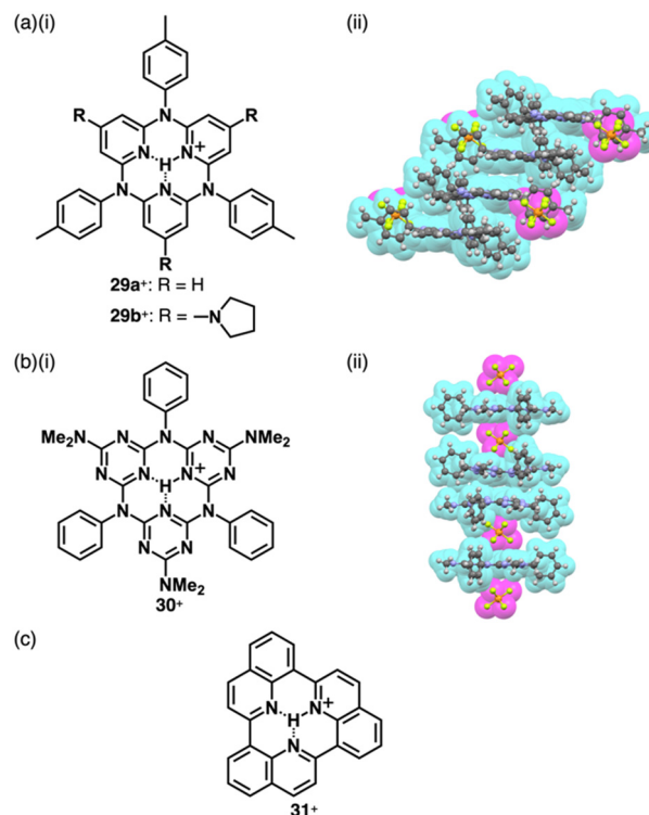
Fig. 19 (a) (i) Protonated azacalix[3](2,6)pyridine 29\text{a},\text{b}^+ and (ii) single-crystal X-ray structure of 29\text{a}^+ \cdot \text{PF}_6^- (redrawn from a cif file: 298963), (b) (i) protonated azacalix[3]triazine 30^+ and (ii) single-crystal X-ray structure of 30^+ \cdot \text{PF}_6^- (redrawn from a cif file: 2072959) and (c) protonated triquinoline 31^+ .
