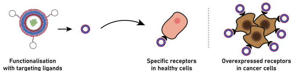
Fig. 14 Active targeting approaches used in therapeutic protein delivery to cancer cells by polymersomes. Targeting ligands such as peptides, sugars as well as small molecules are often conjugated onto the surface of the polymer vesicles to bind to overexpressed receptors commonly found in cancer cells.
