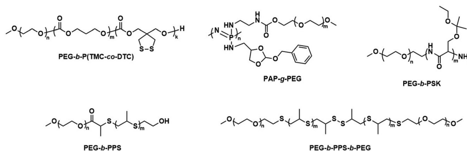
Scheme 6 Chemical structures of stimuli-responsive block copolymers used to create polymersomes for stimuli-responsive disassembly. Polymersomes containing PDTMC form disulfide crosslinks which break in reductive environments, e.g. tumour cytoplasm (Zhong and coworkers 163 ). PAP- g -PEG and PEG- b -PSK polymersomes are pH responsive as ester hydrolysis at pH 5.5 causes a hydrophobic-to-hydrophilic shift and polymersome collapse (Qiu and coworkers, 168 Gu and coworkers 169 ).
