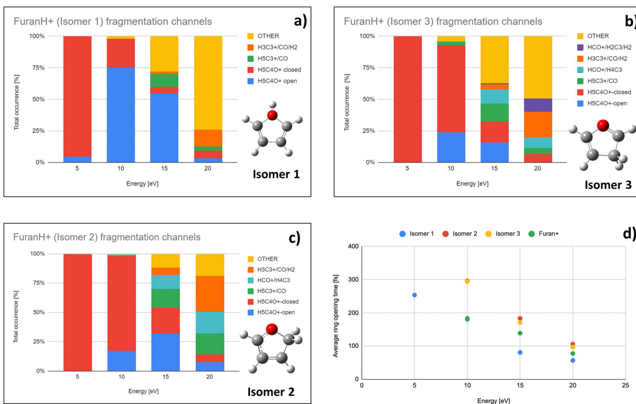
Fig. 10 Molecular dynamics results: (a)–(c) Total occurrence of fragmentation channels as a function of the internal energy of isomer 1, 3 and 2, respectively. Only channels leading to fragments observed in the experiment are explicitly presented. Category OTHER, shown in orange, collects the remaining fragmentation channels. (d) Averaged ring opening times as a function of internal energy.
