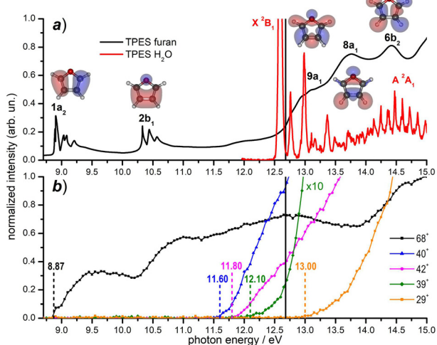
Fig. 2 (a) Threshold photoelectron spectra (TPES) of the neutral furan 56 (black data) and water 59 (red data) molecules from literature data; the corresponding electronic states are also indicated. The Hartree–Fock molecular orbitals of furan are also shown; (b) photoionization yields for the furan radical cation ( 68^+ ) and its fragments (present experiment). Vertical dashed lines indicate the AEs of the ions from literature (see the text). The black solid line in the top and bottom panels indicates the value h\nu = 12.68 eV, at which reactivity experiments have been carried out.
