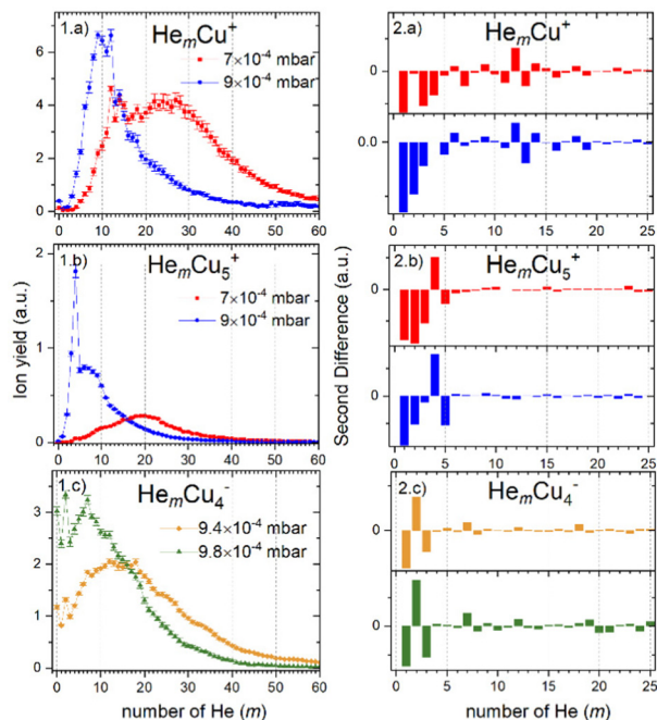
Fig. 2 Left: The cluster size distributions of selected He m Cu n +/- . Plots (1.a) and (1.b) show the cations measured at 7 \times 10^{-4} (red squares) and 9 \times 10^{-4} mbar (blue circles). Plot (1.c) shows the distributions of anions measured at 9.4 \times 10^{-4} (orange diamonds) and 9.8 \times 10^{-4} (green triangles). The symbols represent the ion yield of every m and are complemented with an error bar. Right: The second difference of the selected cluster size distributions of He m Cu n +/- . Plots (2.a) and (2.b) show the cations measured at 7 \times 10^{-4} (red bars) and 9 \times 10^{-4} mbar (blue bars). Plot (2.c) shows the distributions of anions measured at 9.4 \times 10^{-4} (orange bars) and 9.8 \times 10^{-4} (green bars) mbar.
