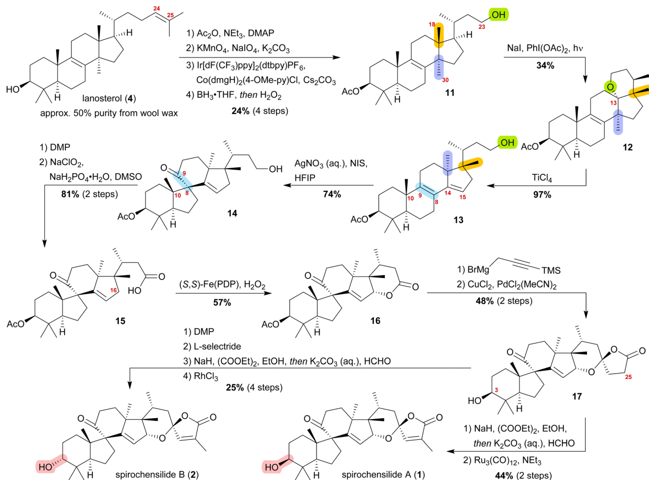
Scheme 2 Semisyntheses of spirochensilide A ( 1 ) and B ( 2 ) by Heretsch and co-workers. ppy = 2-phenylpyridine, dtbbpy = 4,4'-di- t -butyl-2,2'-bipyridine, dmgh = dimethylglyoximate, (S,S)-PDP = (–)-2-((S)-2-((S)-1-(pyridin-2-ylmethyl)pyrrolidin-2-yl)pyrrolidin-1-yl)methylpyridine.
