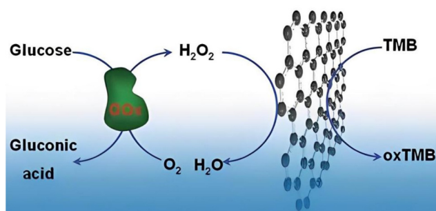
Fig. 11 Schematic diagram of a colorimetric approach for the detection of glucose based on GOx and the GO-COOH catalyzed TMB- \text{H}_2\text{O}_2 system. 122
