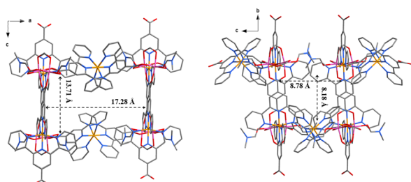
Fig. 2 Stick representation of the Cu-Ru single crystal structure, showing the cds ( 6^5\cdot 8 ) coordination topology.
