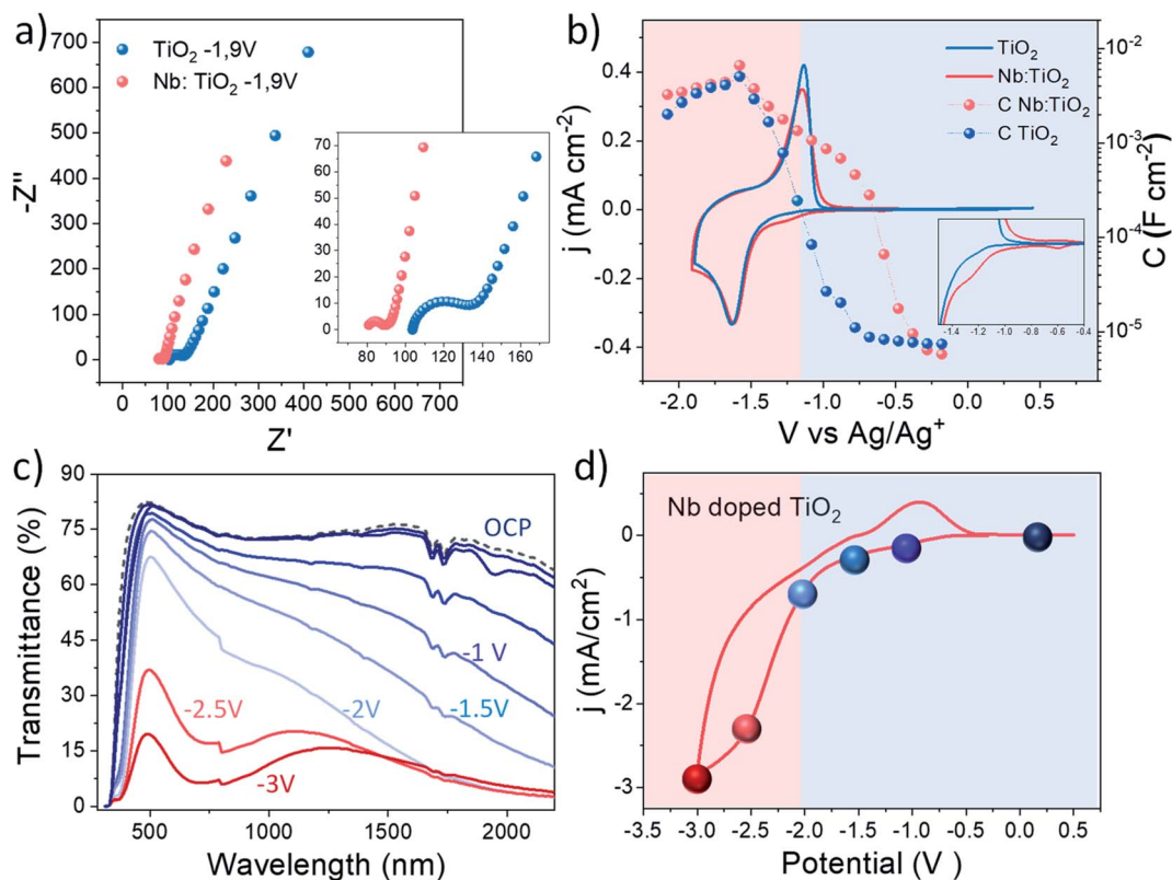
Fig. 5 (a) Nyquist Plot of bare and Nb doped \text{TiO}_2 at -1.9\text{ V vs Ag/Ag}^+ . (b) Cyclic voltammetry (solid lines) and charge capacitance (balls) associated with the different potential points of \text{TiO}_2 (blue) and Nb-doped \text{TiO}_2 (red). (c) Transmittance spectra and (d) cyclic voltammogram of a lab-scale device of Nb doped \text{TiO}_2 at 50\text{ mV s}^{-1} . The spheres represent the potential points at which the transmittance measurements of the device have been carried out.
