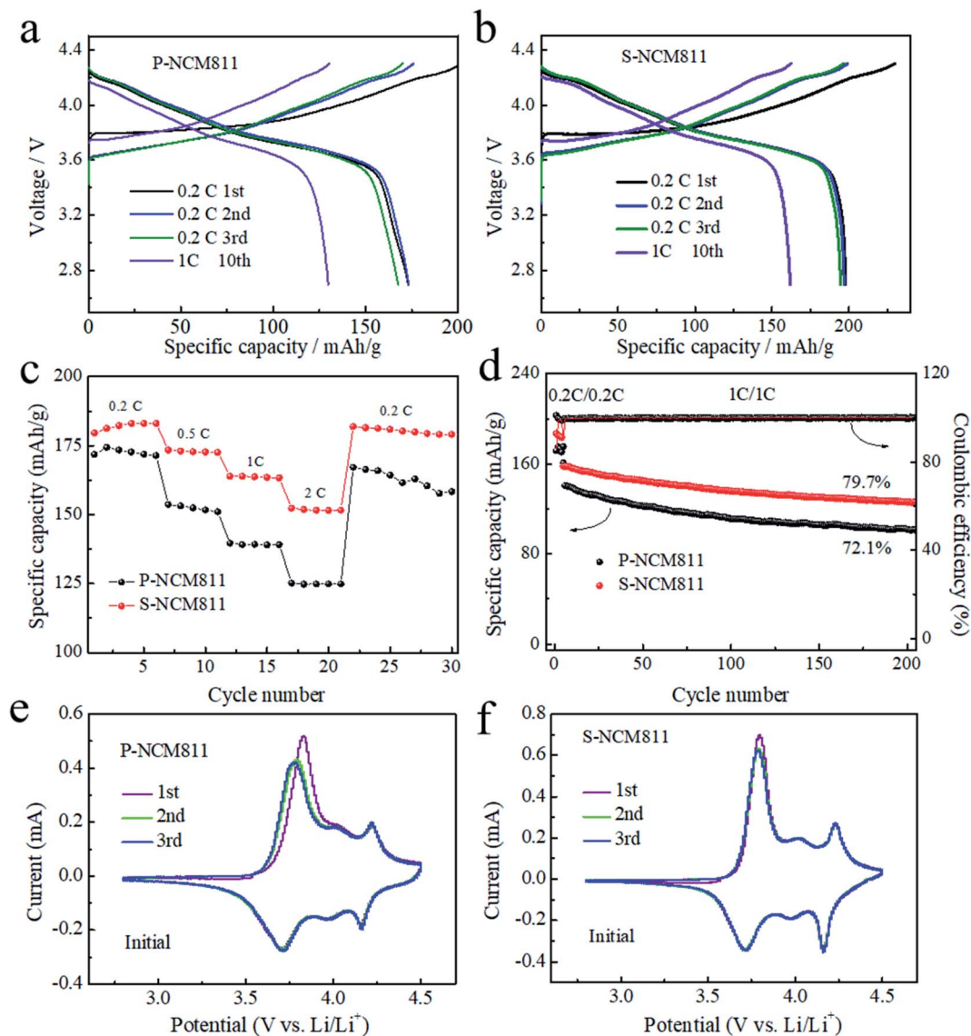
Fig. 3 The charge–discharge curves of (a) P-NCM811 and (b) S-NCM811. (c) Rate and (d) cycling performance. Cyclic voltammery characterization of (e) P-NCM811 and (f) S-NCM811 at the initial state.
