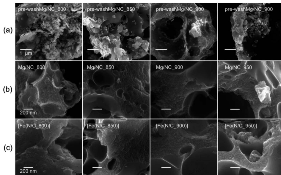
Fig. 1 Scanning electron micrographs of (a) MgO@NC as pyrolyzed, (b) Mg/NiC after washing, (c) [Fe(NiC)] after transmetalation.
