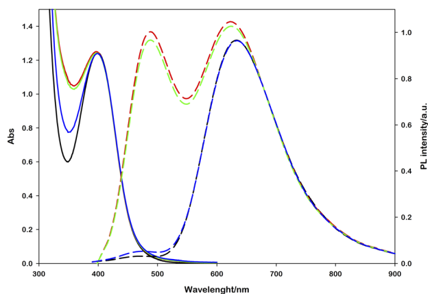
Fig. 5 Absorption (solid lines) and emission (dashed lines) spectral variations observed upon white lamp irradiation and subsequent enzyme assay. Black lines represent the starting reaction mixture, red lines after irradiation (15 hours), green lines upon 15 mM acetaldehyde addition and blue lines after 0.1 μM ADH-1 addition. Emission spectra are obtained upon 340 nm excitation.
