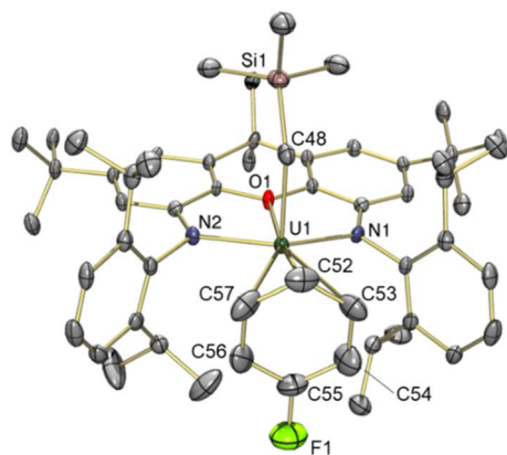
Fig. 6 X-ray crystal structure of [(X A2 )U(CH 2 SiMe 3 )(η 3 -C 6 H 5 F)][B(C 6 F 5 ) 4 ] fluorobenzene ( 5 fluorobenzene), with thermal ellipsoids at 50% probability. Hydrogen atoms, the borate anion, and non-coordinated fluorobenzene lattice solvent are omitted for clarity. Selected bond distances (Å) and angles (°): U(1)–O(1) 2.431(3), U(1)–N(1) 2.215(3), U(1)–N(2) 2.217(3), U(1)–C(48) 2.351(4), U(1)–C(52) 3.126(5), U(1)–C(53) 3.296(5), U(1)–C(54) 3.527(5), U(1)–C(55) 3.594(5), U(1)–C(56) 3.434(5), U(1)–C(57) 3.215(6), U(1)–F(1) 4.528(4), U(1)–C arene ave. 3.37, U(1)–Centroid 3.08, C(55)–F(1) 1.362(7), U(1)–C(48)–Si(1) 134.9(2), O(1)–U(1)–C(48) 89.4(1), N(1)–U(1)–N(2) 127.6(1).
