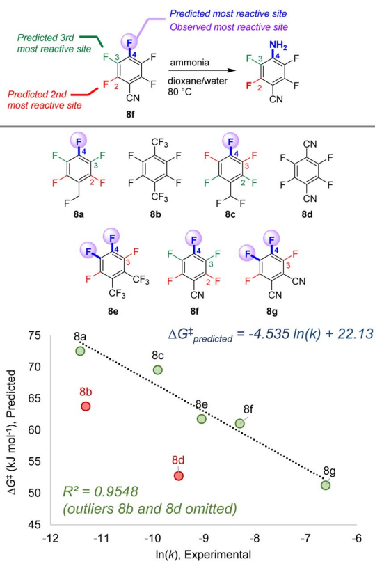
Fig. 8 Site selectivity predictions and rate correlation for \text{S}_{\text{N}}\text{Ar} between fluorinated arenes and ammonia. Experimental data from ref. 99
