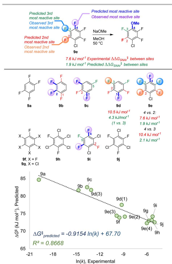
Fig. 9 Site selectivity predictions and rate correlation for \text{S}_{\text{N}}\text{Ar} between fluorinated arenes and methoxide. Experimental data from ref. 100
