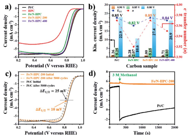
Fig. 6 (a) LSV curves of Pt/C, HPC and Fe/N-HPC, Fe/N-HPC-200 and Fe/N-HPC-400. (b) Electron transfer number, E 1/2 and kinetic current density of Pt/C, Fe/N-HPC, Fe/N-HPC-200 and Fe/N-HPC-400. (c) LSV curves of Pt/C and Fe/N-HPC-200 before and after the accelerated durability test (ADT). (d) Chronoamperometric response of Pt/C and Fe/N-HPC-200 with 3 M methanol at 0.65 V and 1600 rpm. All data are obtained in O 2 -saturated 0.1 M KOH electrolyte.
