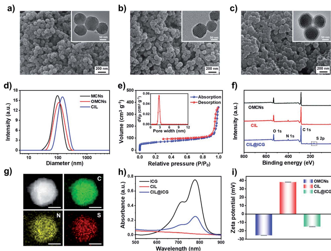
Fig. 1 SEM images of (a) MCNs, (b) OMCNs and (c) CIL; the inset displays the corresponding TEM images. (d) The size distribution of MCNs, OMCNs and CIL. (e) N 2 adsorption–desorption isotherms at 77 K and pore size distribution (inset) curves of CIL@ICG. (f) XPS spectra of OMCNs, CIL and CIL@ICG. (g) High-angle annular dark-field scanning TEM (HAADF-STEM) image and corresponding elemental (C, N, and S) mappings of CIL@ICG. (h) UV-vis-NIR spectra of ICG, CIL and CIL@ICG. (i) Zeta potential of OMCNs, CIL and CIL@ICG.
