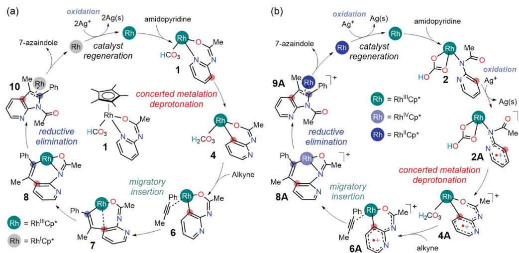
Scheme 2 The mechanism for Rh(III)-catalyzed 7-azaindole synthesis: (a) mechanism adapted from indole synthesis, 17 and (b) oxidatively induced catalytic mechanism (this work).
