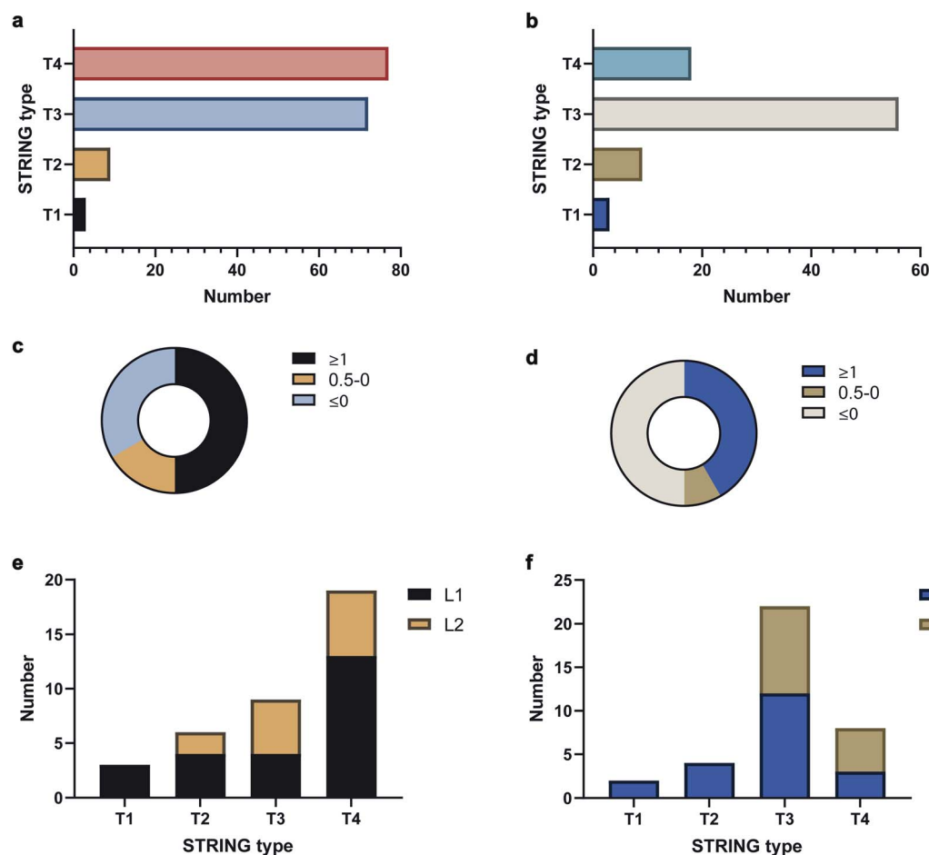
Fig. 3 STRING and AAPL classifications as well as AAPL score distributions of oxidized proteins with anti-ATP1A1 Ab and anti-ERBB2 Ab. (a) STRING type distribution of oxidized proteins with anti-ATP1A1 Ab. (b) STRING type distribution of oxidized proteins with anti-ERBB2 Ab. (c) Percentages of T1 and T2 STRING interactors of ATP1A1 with different AAPL scores. (d) Percentages of T1 and T2 STRING interactors of ERBB2 with different AAPL scores. (e) STRING type distribution of AAPL L1 and L2 interactors of ATP1A1. (f) STRING type distribution of AAPL L1 and L2 interactors of ERBB2.
