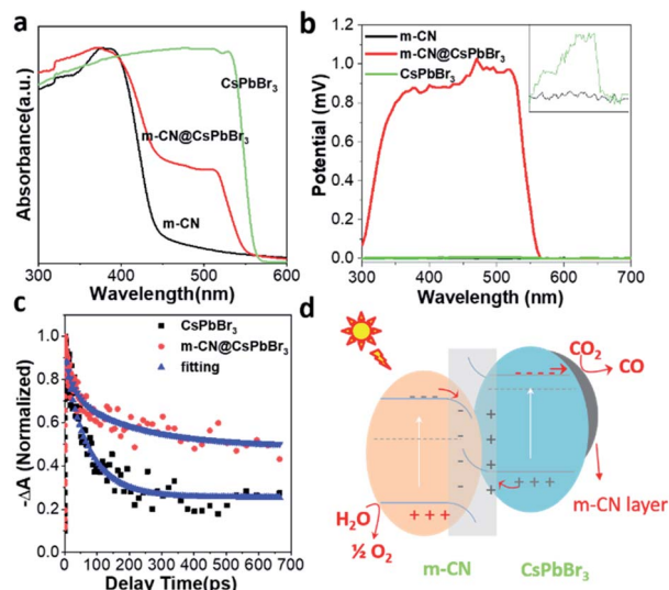
Fig. 2 (a) UV-Vis absorption spectra of m-CN@CsPbBr 3 , the reference m-CN and CsPbBr 3 ; (b) surface photovoltage plots of the m-CN, CsPbBr 3 and m-CN@CsPbBr 3 samples; (c) transient absorption spectroscopy curves and lifetime fittings at 520 nm; (d) band structure of the m-CN@CsPbBr 3 heterojunction and the corresponding paths of CO 2 photo-reduction.
