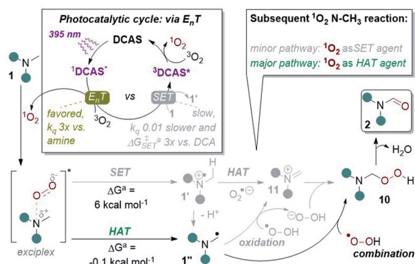
Fig. 10 Proposed reaction mechanism with key experimental and computational evidence. 3 DFT calculations at CAM-B3LYP/6-31++g(2d,p), CPCMC(acetonitrile) level of theory.
