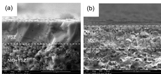
Fig. 23 SEM micrographs showing (a) printed YSZ on Ni-YSZ, and (b) printed SDC on Ni-SDC; post sintering. Reproduced with permission. 90
