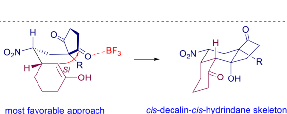
Scheme 21 Synthesis of cis,cis -tricyclic diterpenoid derivatives by a tandem conjugate addition/aldol condensation catalyzed by quinine-derived amine 22 .
