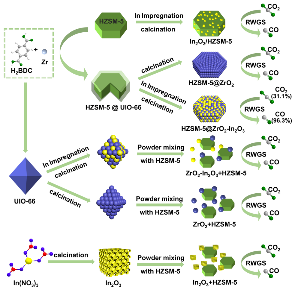
Fig. 1 Assembly diagram of composites (from top to bottom) \text{In}_2\text{O}_3/\text{HZSM-5} , \text{HZSM-5}@ZrO_2 , \text{HZSM-5}@ZrO_2-\text{In}_2\text{O}_3 , ZrO_2-\text{In}_2\text{O}_3 + \text{HZSM-5} , ZrO_2 + \text{HZSM-5} , \text{In}_2\text{O}_3 + \text{HZSM-5} and their effects on \text{CO}_2 hydrogenation.
