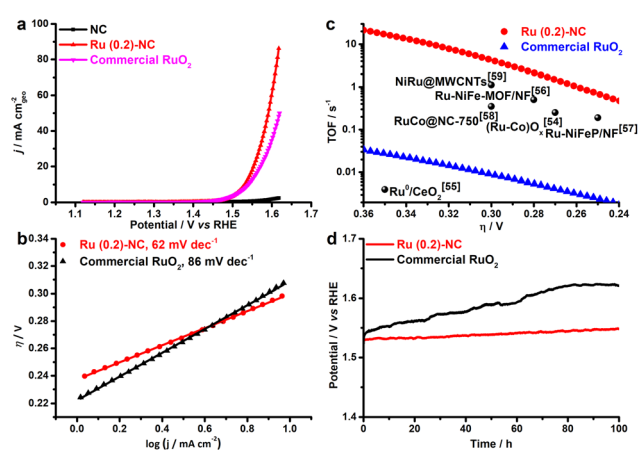
Fig. 3 Electrocatalytic OER performance of Ru (0.2)-NC and other control catalysts. (a) LSV curves. Scan rate: 5 mV \text{s}^{-1} . (b) Tafel slopes. (c) Comparison of the TOF values with other start-of-the-art OER catalysts. (d) Long-term catalytic stability test at 10 mA \text{cm}^{-2} in 1.0 M KOH.
