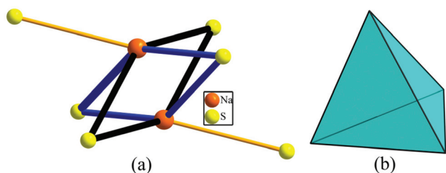
Fig. 5 The center of the unit cell: (a) parallellograms formed by Na and S in 1 ; (b) highly distorted \text{InS}_4 tetrahedron in (\text{K}_3\text{I})[\text{InB}_{12}(\text{InS}_4)_3] .
