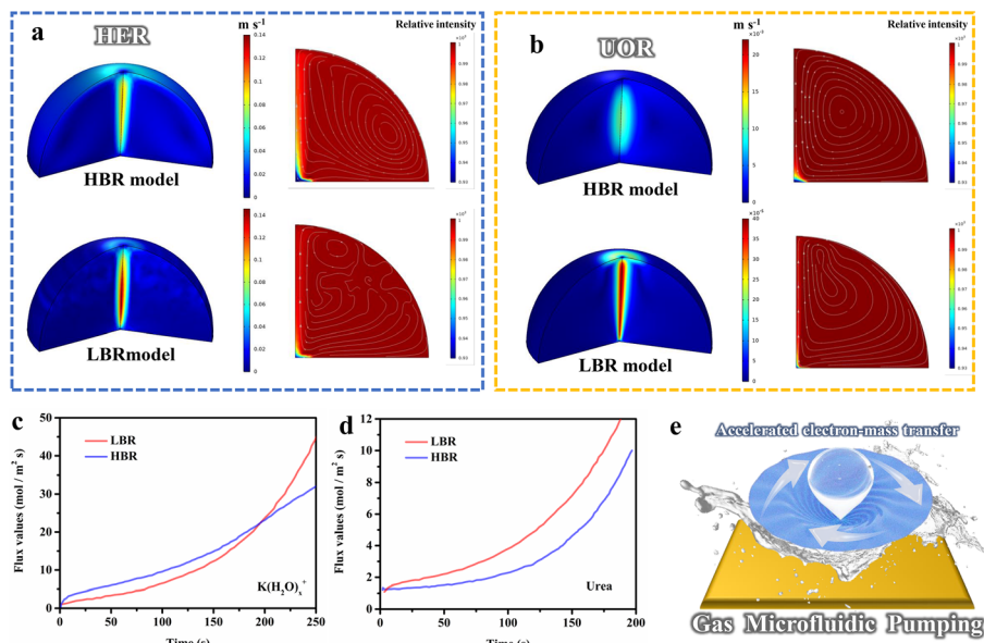
Fig. 6 (a) 3D and corresponding 2D simulation images of the microenvironment flow field states for the HBR and LBR models under the (a) HER and (b) UOR. (c and d) Comparison of the calculated transfer rates. (e) Schematic illustration of the optimal GMP mechanism.
