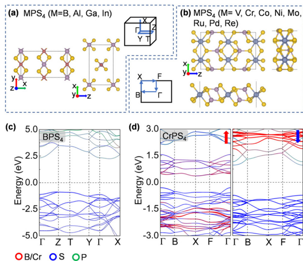
Fig. 5 (a) and (b) Atomic structures of assembled bulk MPS_4 ( M = B, Al, Ga, In ) and an MPS_4 ( M = V, Cr, Co, Ni, Mo, Ru, Pd, and Re ) monolayer, respectively, displayed from different perspectives. The M, P, and S atoms are shown in blue (pink), purple, and yellow colors, respectively. The corresponding Brillouin zones are illustrated. (c) and (d) Electronic band structures of assembled bulk BPS_4 and monolayer CrPS_4 , respectively. The contributions from different atoms or orbitals are shown by color. The Fermi level is shifted to zero (dashed lines).
