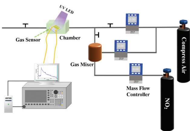
Fig. 2 Schematic diagram of the system for gas-sensing performance tests.
