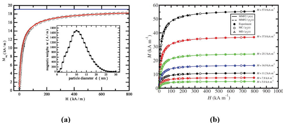
Fig. 23 (a) Equilibrium magnetization M_{\text{eq}} as a function of the internal field H for the ferrofluid AGP 933 of Ferrotec. The horizontal line marks the saturation magnetization M_{\text{sat}} \text{ FF} = 19\,108 \text{ A m}^{-1} . The inset shows the distribution of the magnetic weights w as a function of the magnetic particle diameter d (in nanometers) as deduced from M_{\text{eq}}(H) using Tikhonov's regularization method (reproduced from ref. 377 with permission from Am. Phys. Soc., copyright 2006); (b) complete magnetization curves, M(H) , for ferrofluids of the same set. Filled circles are from experiment, open circles are from MC simulations with p_2(x) , open triangles are from MD simulation with p_2(x) , solid lines are from MMF2 theory with p(x) , and dashed lines (almost coincident with solid lines) are from MMF2 theory with p_2(x) . The statistical uncertainties in the simulation points are smaller than the symbol size; MMF2-second-order modified mean-field theory, MC-Monte Carlo simulation, and MD-molecular dynamics simulation. Reproduced from ref. 378 with permission from Am. Phys. Soc., copyright 2006.
