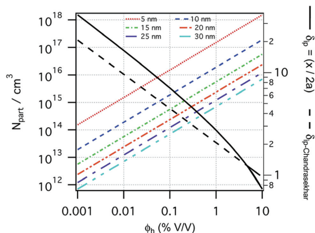
Fig. 5 Number of particles ( N_{\text{part}} ) per cubic centimeter in a ferrofluid and the relative distance ( \delta_{ip} ) between the particle surfaces as a function of the hydrodynamic volume fraction ( \phi_h ), where x is the distance between the particle surfaces and a is the hydrodynamic particle radius, estimated considering a monodisperse particle size distribution, neglecting the influence of Brownian motion, external shear stress, or magnetic field. Particle sizes considered from 5 to 30 nm (reproduced from ref. 161 with permission from Royal Soc. Chem., copyright 2014).
