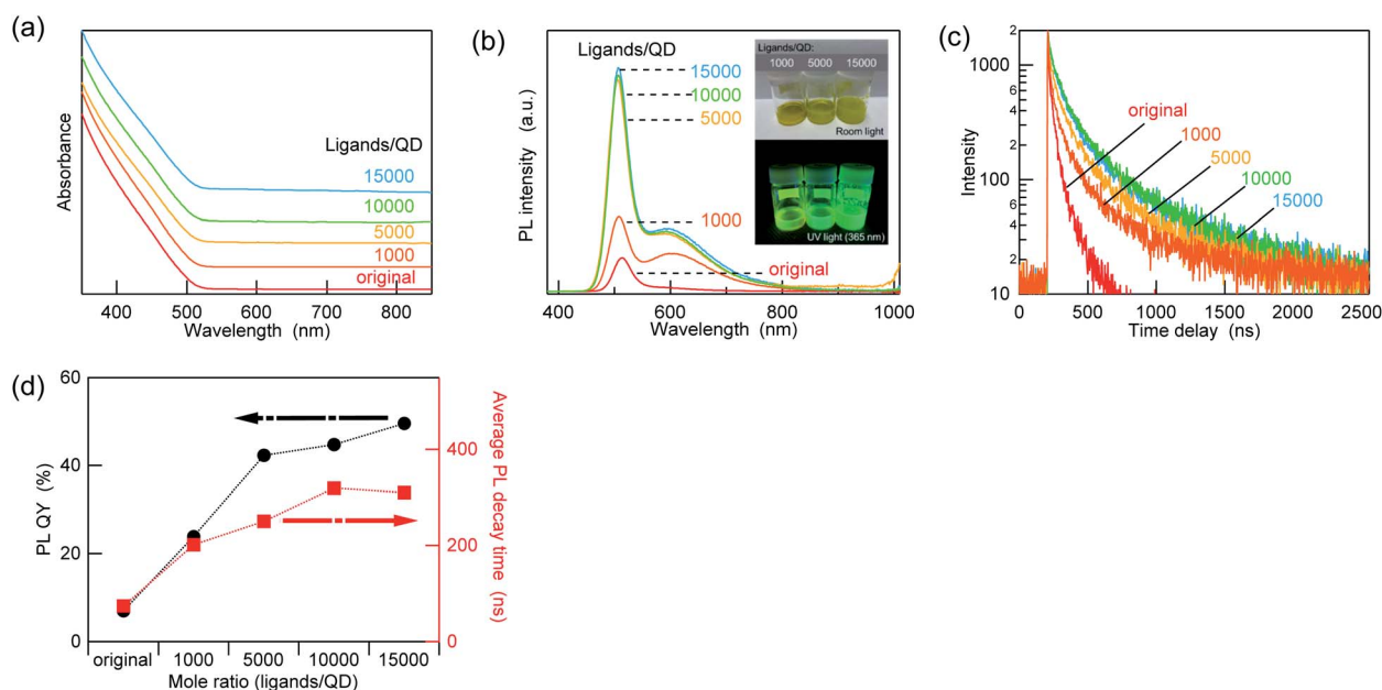
Fig. 6 (a) UV-vis absorption spectra, (b) PL spectra, and (c) PL decay curves of the AIGS/Ga y core/shell-like QDs before and after the treatment with ZnCl 2 at different molar ratios (1000–15 000 ligands/QD). The UV-vis absorption spectra are offset for better clarity, and the insets in (b) shows photographs of the samples under ambient light and UV light. The PL decay curves were recorded at an excitation wavelength of 365 nm and an observation wavelength of 507 nm. (d) Variations in the PL QYs and average lifetimes as a function of the ZnCl 2 amount.
