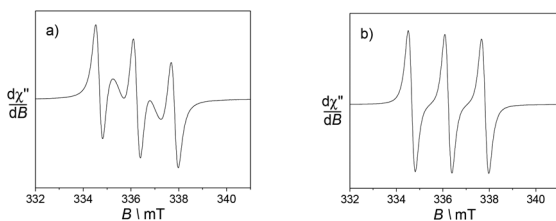
Fig. 4 X band EPR spectra of 0.5 mM \text{CH}_3\text{CN} solutions of the ligands (a) \text{L}_1 and (b) \text{L}_2 . Microwave freq. 9.42 GHz; power, 3.5 mW; modulation amp., 0.2 mT; freq. 100 KHz. T = 293 K.
