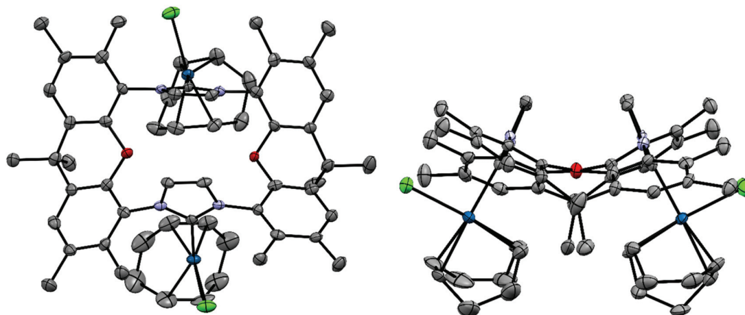
Fig. 1 X-ray crystal structure (thermal ellipsoids 80%) of [(\text{IrCl}(\text{cod}))_2(\mathbf{9})] (colour code: Ir blue, Cl green, O red, N blue, H not displayed) plots: perpendicular to xanthenes plane and along the oxygen–oxygen axis. Important distances (pm), bond lengths (pm) and angles ( ^\circ ): Ir...Ir 702.4, Ir–C (NHC) 205.0(6), 206.1(6), Ir–Cl 238.0(2), 238.1(2), Ir–C(cod) 210.7(6), 214.2(7), 215.0(6), 219.7(7) (av. 214.9), 209.6(6), 211.4(7), 215.7(8), 220.3(8) (av. 214.3), Cl–Ir–C(NHC) 91.8(2), 92.3(2), C(NHC)–Ir–C(cod) 173.6(3), 173.1(3) and 149.9(2), 149.1(2).
