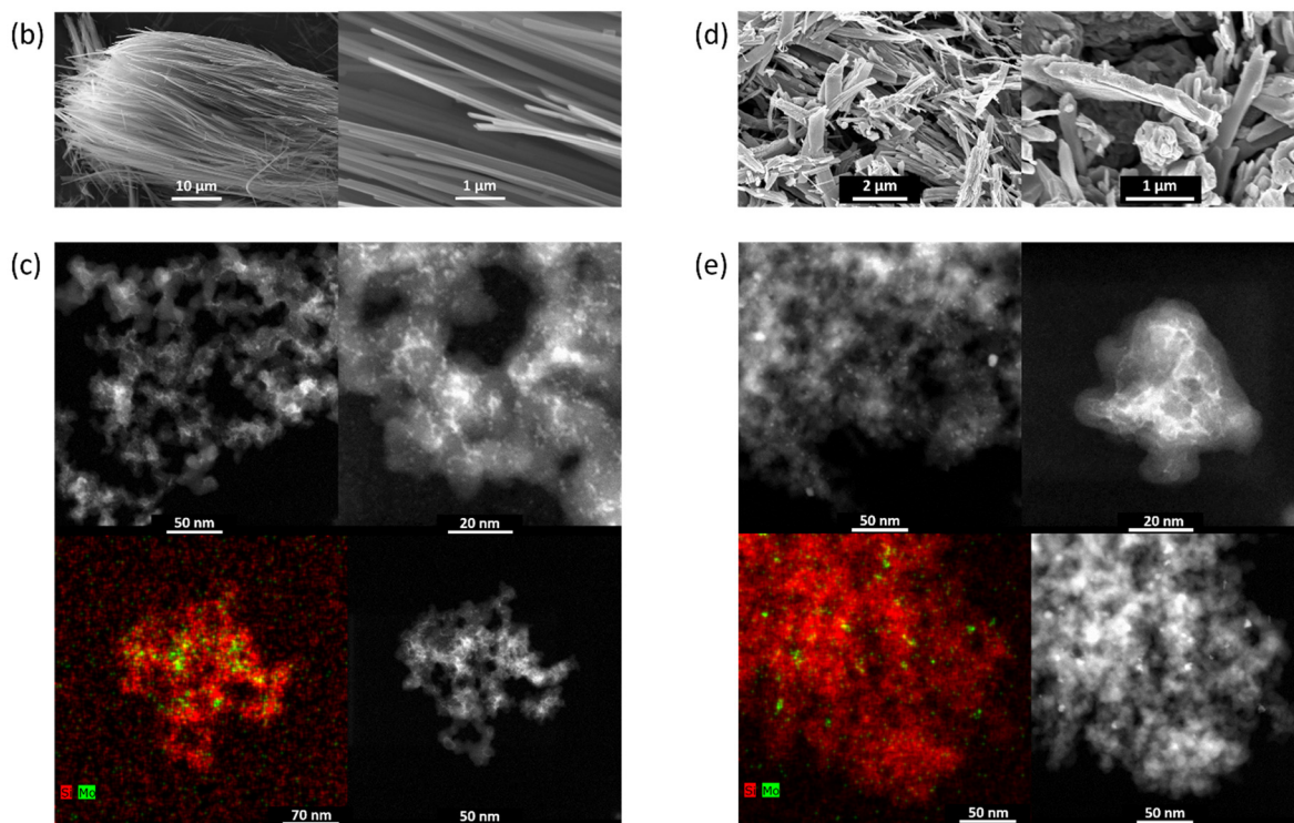
Fig. 1 a) Synthesis of \text{Mo}_2\text{C-nb} from \alpha\text{-MoO}_3\text{-nb} and \text{Mo}_2\text{C/SiO}_2 from silica-supported delaminated \text{MoO}_3 films \text{MoO}_3/\text{SiO}_2 ; b) SEM images of as synthesized \alpha\text{-MoO}_3\text{-nb} ; c) HAADF-STEM images and EDX elemental (Si and Mo) maps of \text{MoO}_3/\text{SiO}_2 ; d) SEM images of \text{Mo}_2\text{C-nb} ; and e) HAADF-STEM images and EDX maps of \text{Mo}_2\text{C/SiO}_2 .
