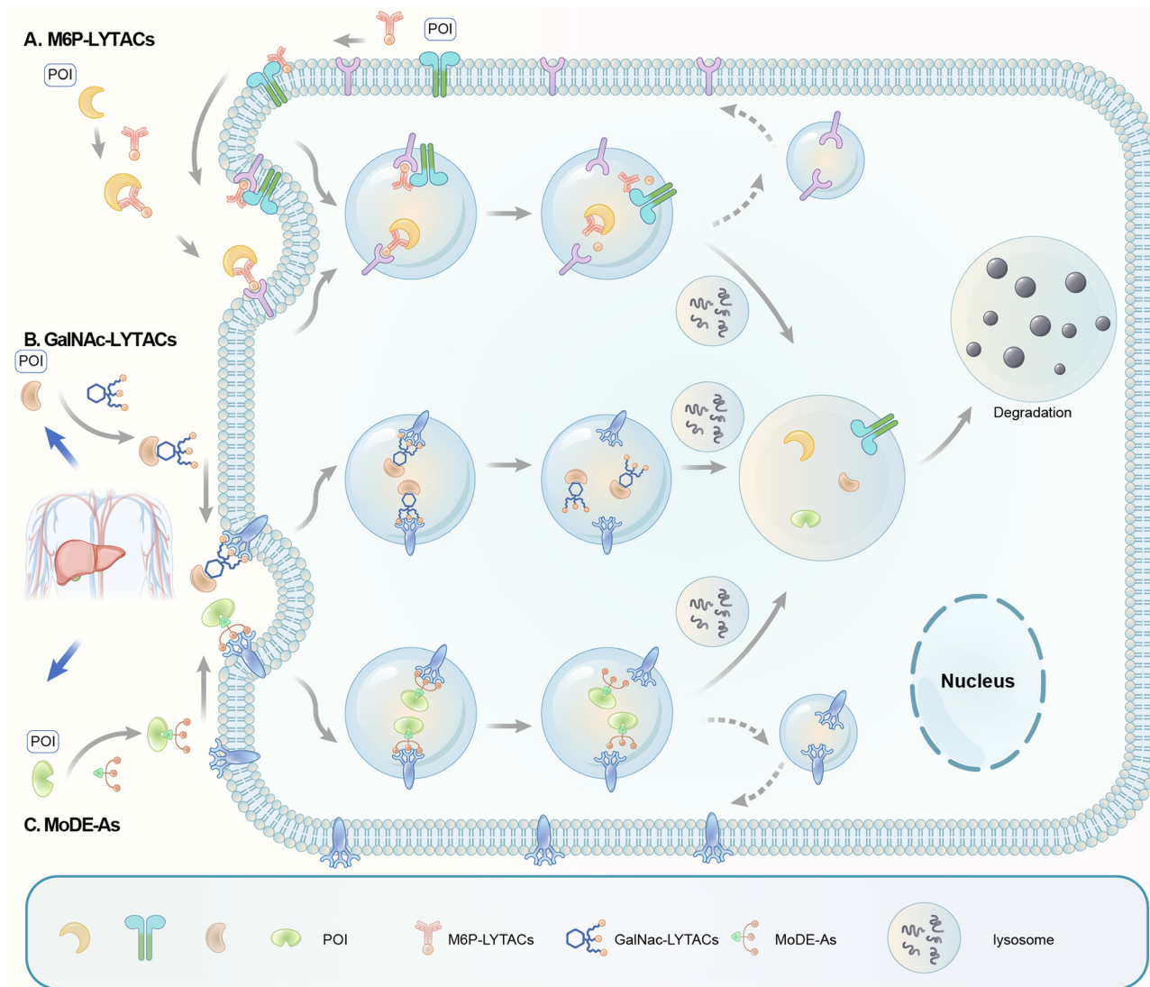
Fig. 22 Illustration of degrader technologies engaging the endosomal–lysosomal pathway. (A) M6P-LYTACs: M6P-LYTACs utilize a glycan tag binding with Cl-M6PR to mark extracellular or transmembrane POI for intracellular lysosomal degradation following receptor-mediated internalization; (B) GalNAc-LYTACs & (C) MoDE-As utilize a glycan tag binding with the liver-specific ASGPR to mark POI for intracellular lysosomal degradation following receptor-mediated internalization.
