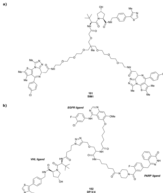
Fig. 43 Trivalent PROTACs. Trivalent degrader SIM1 (101) targeting both BDs of Brd4 via two incorporated BET ligands (a), 187 and trivalent degrader DP-V-4 (102) simultaneously targeting EGFR and PARP proteins (b). 189
