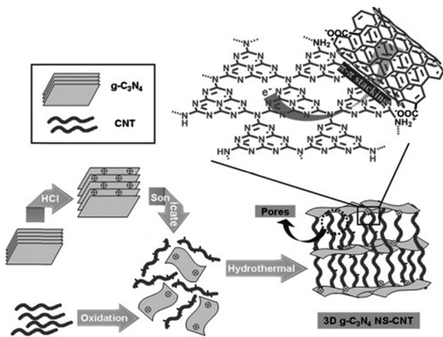
Fig. 100 Fabrication of the 3D g-C 3 N 4 NS-CNT porous composite. Reproduced with permission from ref. 1410. Copyright Wiley 2014.
