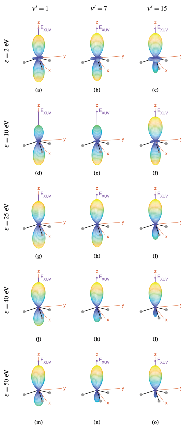
Fig. 7 Vibrationaly resolved MFPADs for oriented molecules (in 0+ initial state) at room temperature, ammonia's valence shell and an ionizing pulse linearly polarized in the z axis of the MF. All MFPADs are renormalized, the real scale can be seen approximately in Fig. 4.
