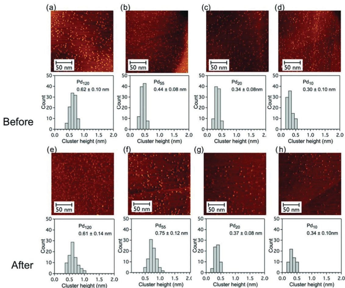
Fig. 3 Constant current STM images ( 200 \times 200 \text{ nm}^2 , 0.4 nA, 0.4 V) of graphite-supported size-selected \text{Pd}_N clusters ( N = 120, 55, 20 and 10, low coverage) and histograms of the cluster height distributions before and after catalytic reaction at reactant ratio of \text{C}_6\text{H}_{12}:\text{O}_2 = 1:10 ; (a–d) as-deposited clusters before catalytic measurements and (e–h) after reaction catalytic measurements. The mean height of the cluster is given in each case. Adapted from ref. 103 with permission from Taylor & Francis.
