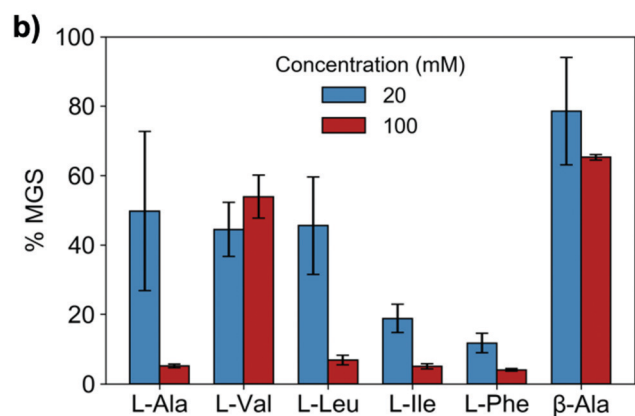
Fig. 1 IRI activity of amino acids. (a) Chemical structures and calculated logP and surface area normalised logP; (b) IRI activity of amino acids. n = 3 , +/- S.D. MGS = mean grain size.
