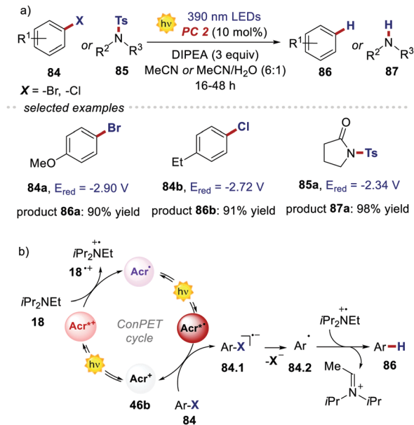
Scheme 40 (a) Reductive dehalogenation of aryl halides ( 81 ) and reductive desilylation of amines ( 82 ) triggered by the excited radical acridinium Acr^{\bullet+} 41b . (b) The proposed mechanism for the dehalogenation of arenes.
