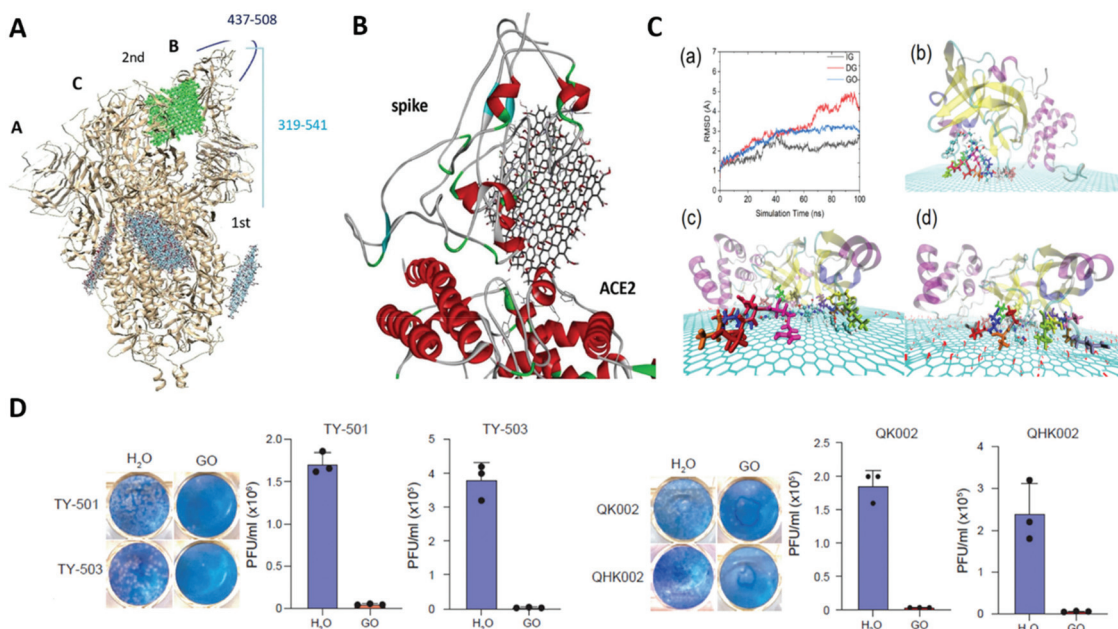
Fig. 12 Anti-SARS-CoV-2 activity of 2D nanosheets. (A) Binding of GO at different sites of open state of spike protein (6VYB). (B) Binding of GO with spike-ACE2 complex (6M0J) with binding affinity -9.1 \text{ kcal mol}^{-1} . Reproduced with permission. Copyright 2021, Wiley. 264 (C) Deactivation of the SARS-CoV-2 protease M Pro by GO. (a) RMSD of the active pocket of M Pro for all systems during 100 ns MD simulations. Representative snapshots of M Pro adsorbed onto (b) IG, (c) DG, and (d) GO. Reproduced with permission. 265 Copyright 2021, American Chemical Society. (D) Anti-SARS-CoV-2 activity against Brazilian strains (TY7-501 and TY7-503) and U.K. strains (QK002 and QHN001) in the presence and absence of GO ( 100 \mu\text{g mL}^{-1} ) using plaque assay. Reproduced with permission. 267 Copyright 2021, American Chemical Society.
