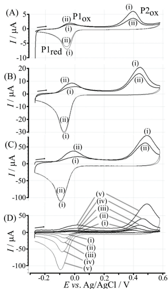
Fig. 7 Cyclic voltammograms (scan rate (A) 10 , (B) 50 , (C) 200 \text{ mV s}^{-1} , (D) overlay for (i) 10 , (ii) 25 , (iii) 50 , (iv) 100 , and (v) 200 \text{ mV s}^{-1} ) for a 6 \mu\text{g} T1-functionalised electrode with poly-NHG introduced onto the surface and immersed in phosphate buffer (0.1 M, pH 7).
