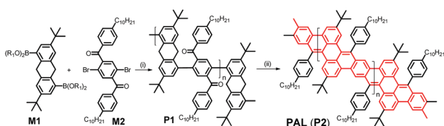
Scheme 2 Synthesis of a conjugated hydrocarbon ladder polymer PAL (P2) with a polyacene skeleton; the boronic esters are preferably pinacolates ( R_1 – R_2 : CMe_2 – CMe_2 ); (i) Pd(PPh_3)_4 , K_2CO_3 , toluene/ H_2O , (ii) KOC(CH_3)_3 /DMF.
