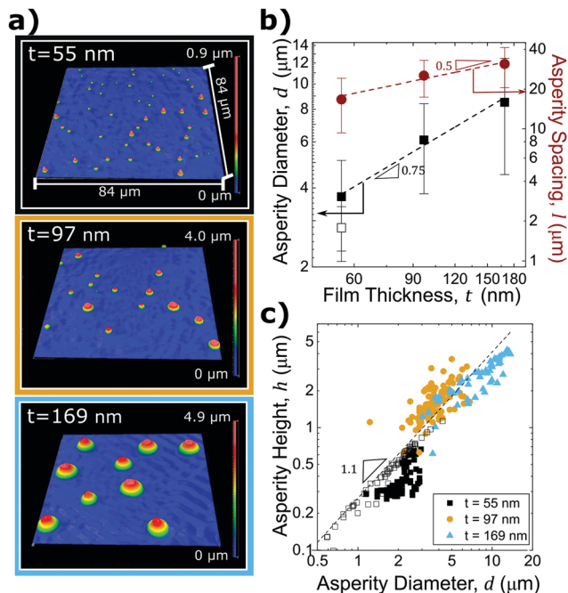
Fig. 2 (a) Optical profilometry images of the dewetted PS asperities. (b) Feret diameter, d and asperity spacing, l as a function of film thickness, t . The error bars represent one standard deviation. (c) Asperity height, h , as a function of d . Note that the scales in (b) and (c) are logarithmic. Filled symbols represent data collected by optical profilometry and open symbols represent data collected by AFM. The sample size used for each asperity size in plots (b) and (c) is n \geq 75 .
