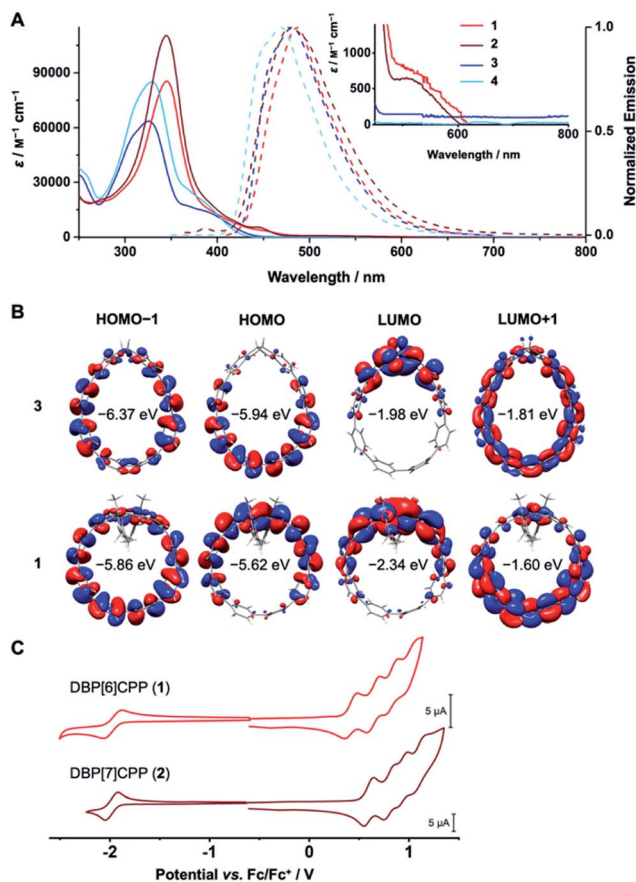
Fig. 4 (A) Absorption ( 10^{-5} to 10^{-6} M) and emission spectra ( 10^{-6} to 10^{-7} M) of 1–4 in \text{CH}_2\text{Cl}_2 ; (B) frontier molecular orbitals of 3 and 1 (PW6B95–D3(BJ)/def2–TZVP//PBEh–3c); (C) cyclic voltammograms of 1 and 2 (negative potential range in THF, positive in \text{CH}_2\text{Cl}_2 , 1 mM concentration, 0.1 M n\text{-Bu}_4\text{NPF}_6 , scan rate 0.2 \text{ V s}^{-1} , glassy carbon electrode, potentials plotted vs. \text{Fc}/\text{Fc}^+ as internal standard).
