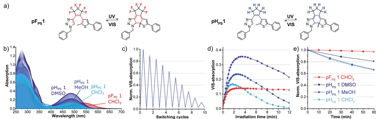
Fig. 7 Comparison of triazole photoswitches with perfluorinated ( \text{pF}_{\text{Ps}} \mathbf{1} ) and perhydrogenated ( \text{pH}_{\text{Ps}} \mathbf{1} ) cyclopentene bridge: (a) structures of the respective OF and CF isomers, (b) time-dependent changes in the absorption spectra upon UV light irradiation (310 nm, 60 \mu\text{M} conc.) to the (p)PSS, (c) reversibility of \text{pH}_{\text{Ps}} \mathbf{1} in methanol, (d) kinetic trace of the VIS absorption bands (CF isomers) during extended UV light irradiation, (e) thermostability (20 ^{\circ}\text{C} ), see also Table S4.†
