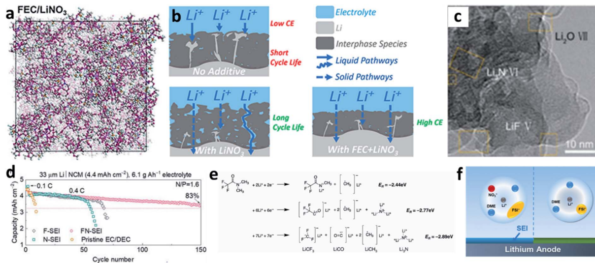
Fig. 11 Constructing F-rich and N-rich composite interfaces for stabilizing Li metal electrodes. (a) MD results for a carbonate electrolyte with FEC as the solubilizer to improve the solvability of \text{LiNO}_3 ; reproduced with permission. Copyright 2018, John Wiley and Sons. (b) Schematic illustration of the formation of a denser and more effective SEI on the Li metal electrode due to the synergistic effects of FEC and \text{LiNO}_3 in the electrolyte; reproduced with permission. Copyright 2019, American Chemical Society. (c) Cryo-TEM image of the SEI formed in the electrolyte with tris(pentafluorophenyl)borane and \text{LiNO}_3 as a dual additive; reproduced with permission. Copyright 2020, John Wiley and Sons. (d) Cycling performance of Li-NCM batteries with different types of SEIs; reproduced with permission. Copyright 2020, John Wiley and Sons. (e) Decomposition routes of the FDMA solvent to form \text{Li}_3\text{N} ; reproduced with permission. Copyright 2020, Springer Nature. (f) Structural illustration of the \text{Li}^+ solvation structure of an ether electrolyte with or without \text{NO}_3^- ; reproduced with permission. Copyright 2019, American Chemical Society.
