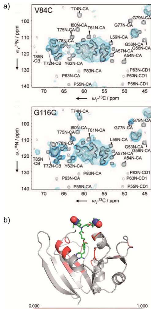
Fig. 7 (a) 800 MHz low-temperature DNP 2D NCA of U- ^{13}\text{C} , ^{15}\text{N} ] spectra (blue) of KcsA mutants V84C (top) and G116C (bottom), spin labeled with AMUPol-MTSSL (see Fig. 1d), compared to room temperature 700 MHz solid-state NMR spectra (black) of wild-type KcsA (black). The presence of the spin label in the mutants leads to paramagnetic bleaching at cryogenic temperature. Reproduced with permission from ref. 67. Copyright 2015 WILEY-VCH Verlag GmbH & Co. KGaA, Weinheim. (b) Model of the protein DHFR complexed with the high affinity ligand TMP derivatized with TOTAPOL (see as well Fig. 3b), with heat map showing the bleaching information obtained from low temperature DNP spectra. The strongest reduction in signal intensity (in red) is observed for residues proximal to the TMP-radical binding pocket. Reproduced with permission from ref. 66. Copyright (2017) American Chemical Society.
