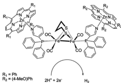
Fig. 22 The photo active species of an [FeFe]-hydrogenase mimic bears two different chromophores. Used with permission from ref. 109.
