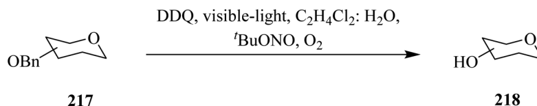
Scheme 76 DDQ-assisted oxidative debenylation of benzyl ethers under visible-light irradiation.
